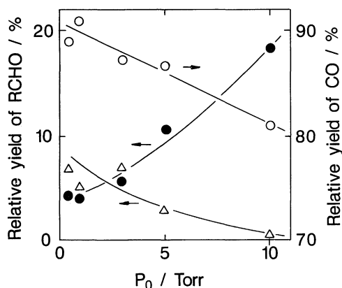
Fig. 4. Effects of P_0 on yield of an oxygen-containing products relative to total yield of all oxygen-containing products. CO (○), H_2CO (●), and CH_3CHO (△). For experimental conditions see the caption in Fig. 2.
